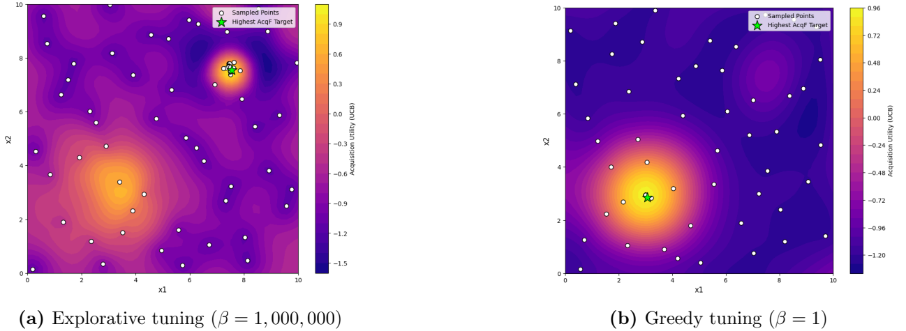
Figure 3: Comparison of the Upper Confidence Bound (UCB) acquisition function behaviour under different exploration parameters ( \beta ). (a) A high \beta value successfully prioritises exploration, identifying a secondary hidden peak. (b) A low \beta value results in overly greedy exploitation, causing the model to stagnate on a single local optimum and ignore unexplored regions.
