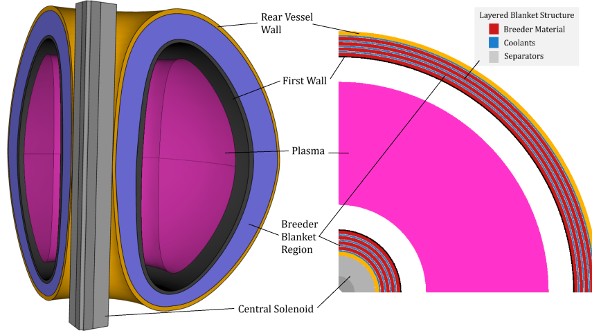
Figure 1: Representative geometry of the simplified Tokamak model generated via Paramak. The simulation domain comprises a 90^\circ revolution with periodic boundary conditions. Included is an example breakdown of the layered blanket, only the coolant and breeder thicknesses are adjusted in this study.
