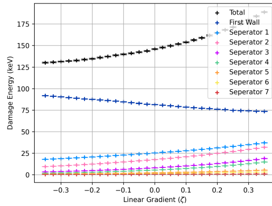
Figure A3: Total damage energy deposited into the plasma-facing first wall and internal structural separators across the geometric gradient.
